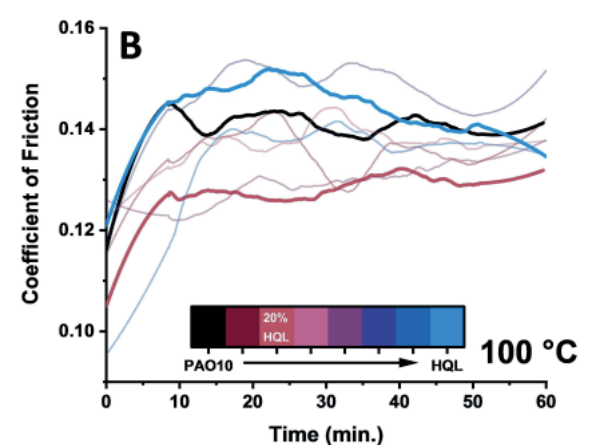
Figure 5. COF of PAO10 and HQL Concentrations at 100oC[10]
