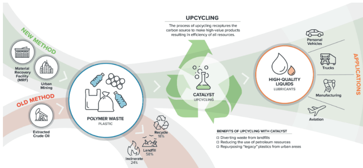
Figure 1. Chemical Recycling Methods: Downcycling and Upcycling[10]
