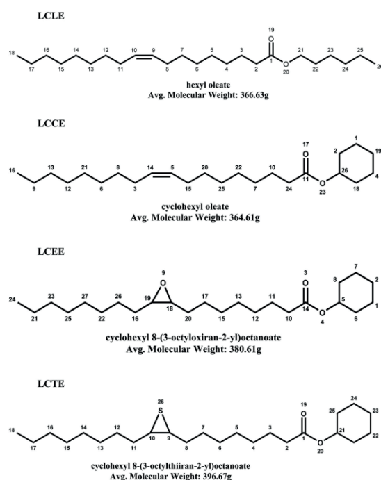
Figure 6. Chemical Structures of Synthesized Esters[11]
