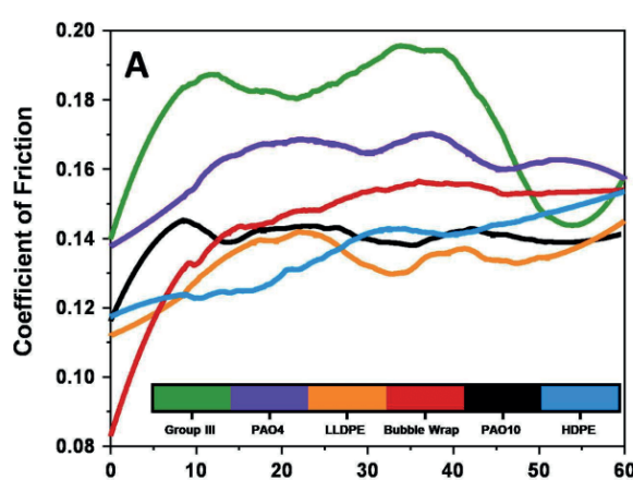
Figure 2. COF Changes at 300oC for Group III, PAO4, LLDPE, Bubble Wrap, PAO10, and HDPE[10]
