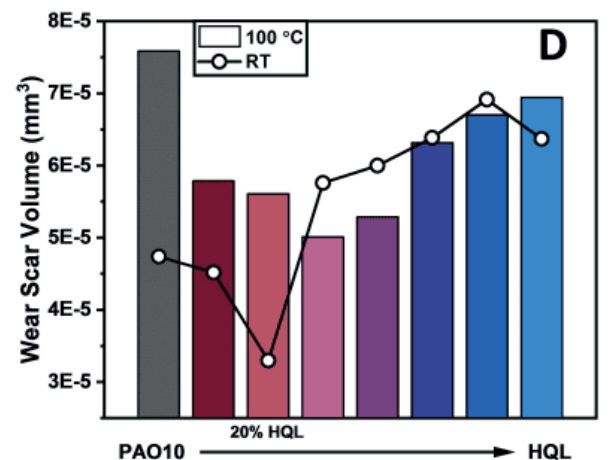
Figure 3. Wear Scar Volumes of PAO10 and HQL Concentrations [10]
