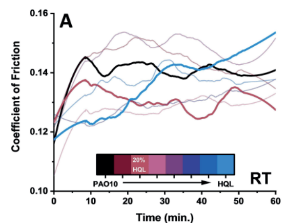
Figure 4. COF of PAO10 and HQL Concentrations at 25oC[10]
